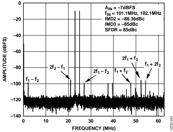
Figure 28. Two-Tone 32k FFT with f_{IN1} = 100.1 MHz and f_{IN2} = 102.1 MHz, f_{SAMPLE} = 125 MSPS, V_{REF} = 1.4 V
