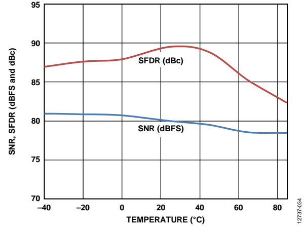
Figure 31. SNR, SFDR vs. Temperature; f_{IN} = 9.7 MHz, f_{SAMPLE} = 125 MSPS, V_{REF} = 1.4 V
