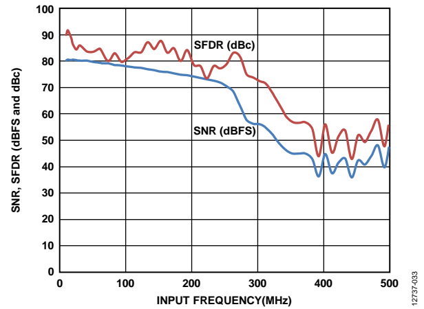
Figure 30. SNR, SFDR vs. Input Frequency ( f_{IN} ); f_{SAMPLE} = 125 MSPS, V_{REF} = 1.4 V
