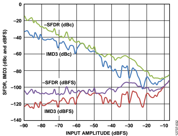
Figure 29. Two-Tone SFDR, IMD3 vs. Input Amplitude ( A_{IN} ) with f_{IN1} = 100.1 MHz and f_{IN2} = 102.1 MHz, f_{SAMPLE} = 125 MSPS, V_{REF} = 1.4 V
