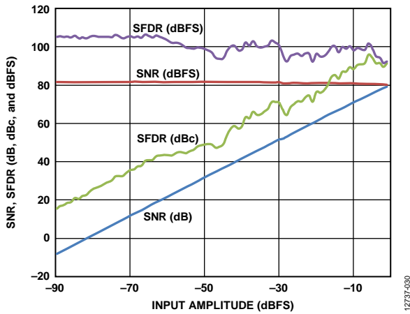
Figure 27. SNR, SFDR vs. Input Amplitude; f_{IN} = 9.7 MHz, f_{SAMPLE} = 125 MSPS, V_{REF} = 1.4 V
