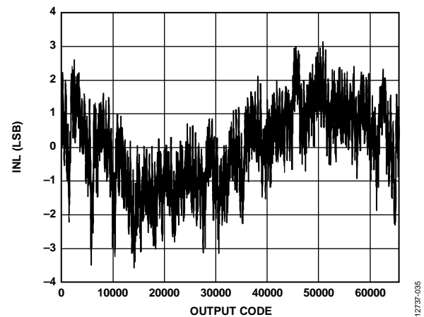
Figure 32. INL; f_{IN} = 9.7 MHz, f_{SAMPLE} = 125 MSPS, V_{REF} = 1.4 V
