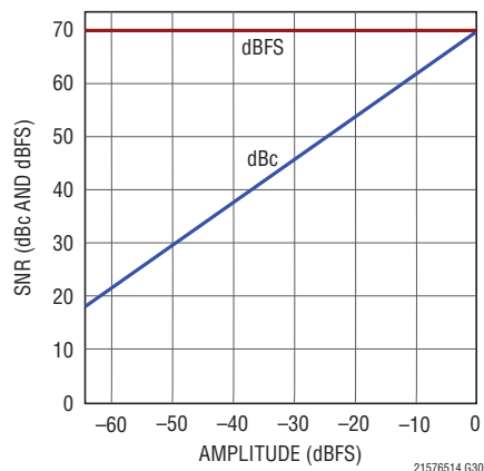
LTC2156-14: SNR vs Input Level, f_{IN} = 70\text{MHz} , 210Mps
