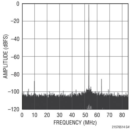
LTC2155-14: 32K Point FFT, f_{IN} = 225\text{MHz} , -1\text{dBFS} , 170Mps
