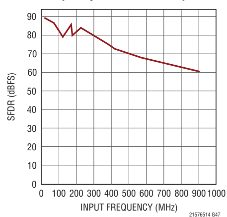
LTC2155-14: SFDR vs Input Frequency, -1\text{dBFS} , 170Mps
