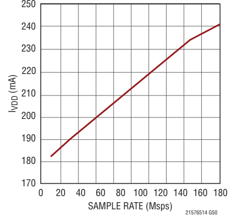
LTC2155-14: I_{VDD} vs Sample Rate, 15MHz Sine Wave Input, -1dBFS
