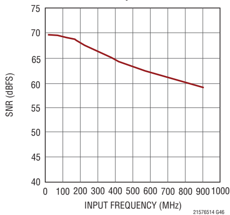
LTC2155-14: SNR vs Input Frequency, -1\text{dBFS} , 170Mps
