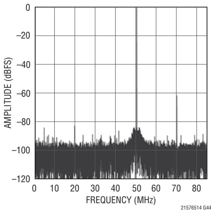
LTC2155-14: 32K Point FFT, f_{IN} = 907\text{MHz} , -1\text{dBFS} , 170Mps
