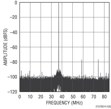
LTC2155-14: 32K Point FFT, f_{IN} = 380\text{MHz} , -1\text{dBFS} , 170Mps
