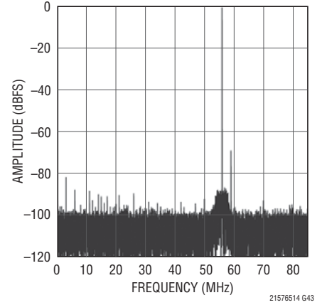
LTC2155-14: 32K Point FFT, f_{IN} = 571\text{MHz} , -1\text{dBFS} , 170Mps
