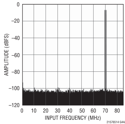
LTC2155-14: 32K Point 2-Tone FFT, f_{IN} = 70.5\text{MHz} and 69.5\text{MHz} , 170Mps
