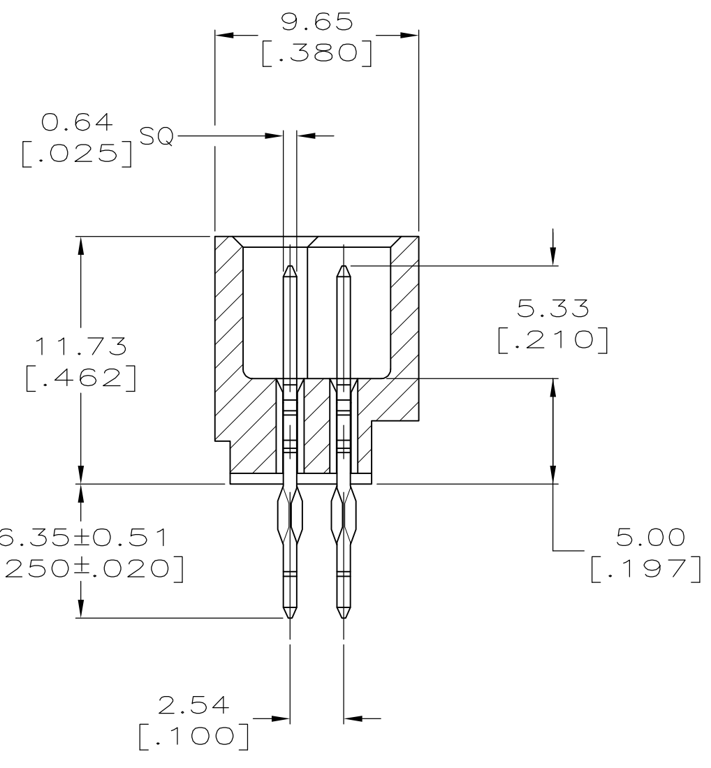
SECTION T-T
