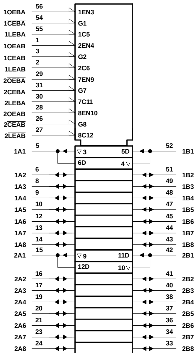
LOGIC SYMBOL (1)
