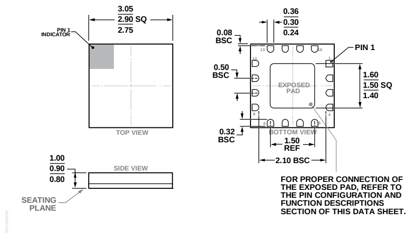
Figure 16. 16-Terminal Ceramic Leadless Chip Carrier [LCC] (E-16-1)
