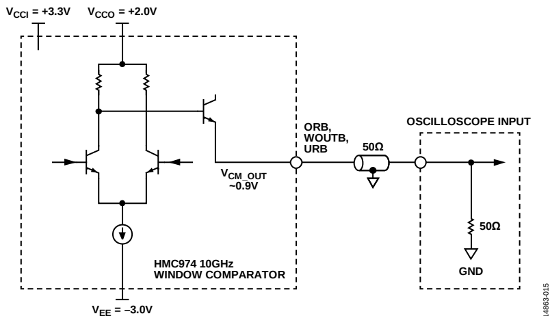
Figure 15. Typical Application Circuit
