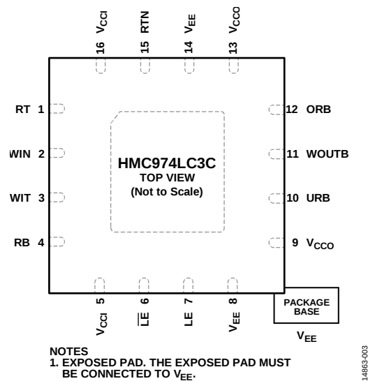
Figure 3. Pin Configuration
