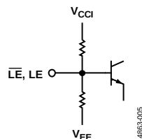
Figure 5. Interface Schematic for LE and \overline{LE}
