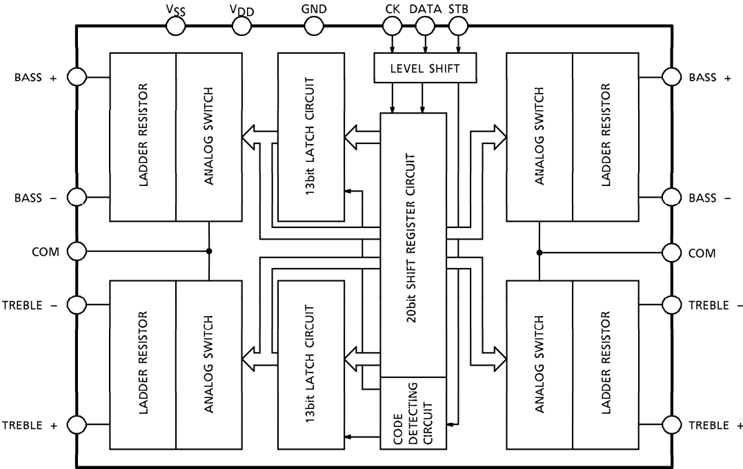
BLOCK DIAGRAM TC9184AP
