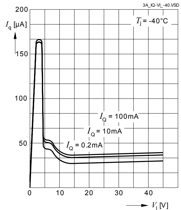
Current Consumption I_q versus Input Voltage V_i at T_j=-40^\circ C (EN=ON)
