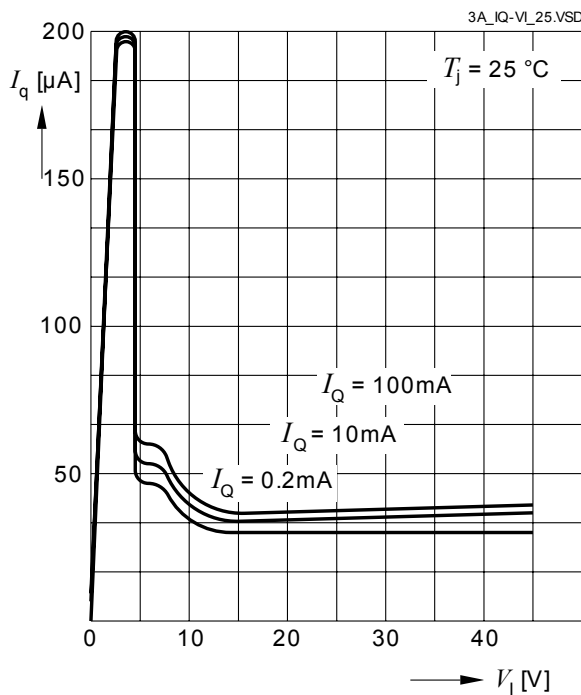
Current Consumption I_q versus Input Voltage V_i at T_j=25^\circ C (EN=ON)
