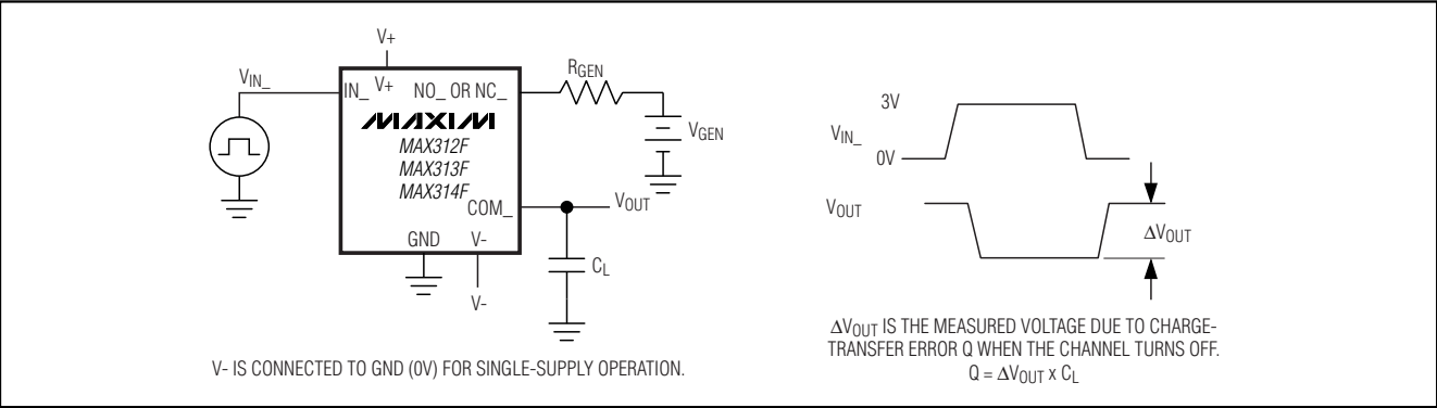
Figure 4. Charge Injection
