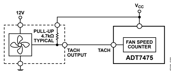
Figure 36. Fan with TACH Pull-Up to V CC
