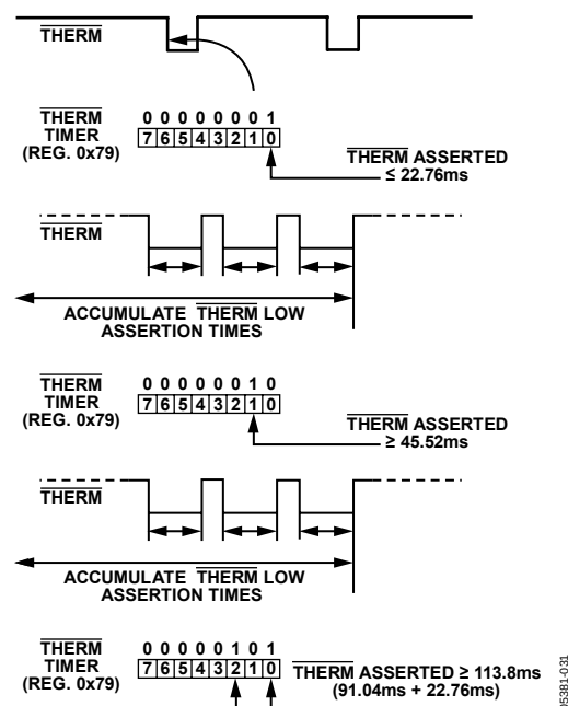
Figure 28. Understanding the \overline{\text{THERM}} Timer
