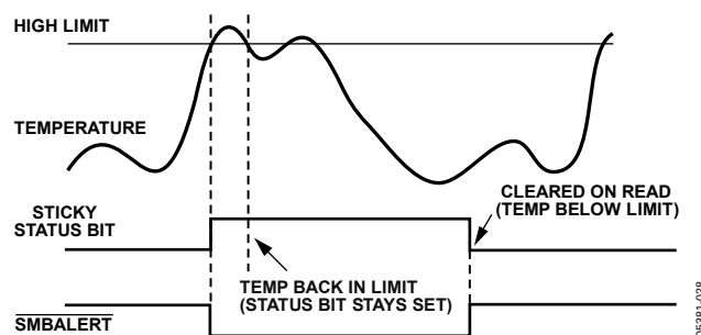
Figure 25. SMBALERT and Status Bit Behavior
