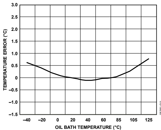
Figure 11. Internal Temperature Error vs. ADT7475 Temperature
