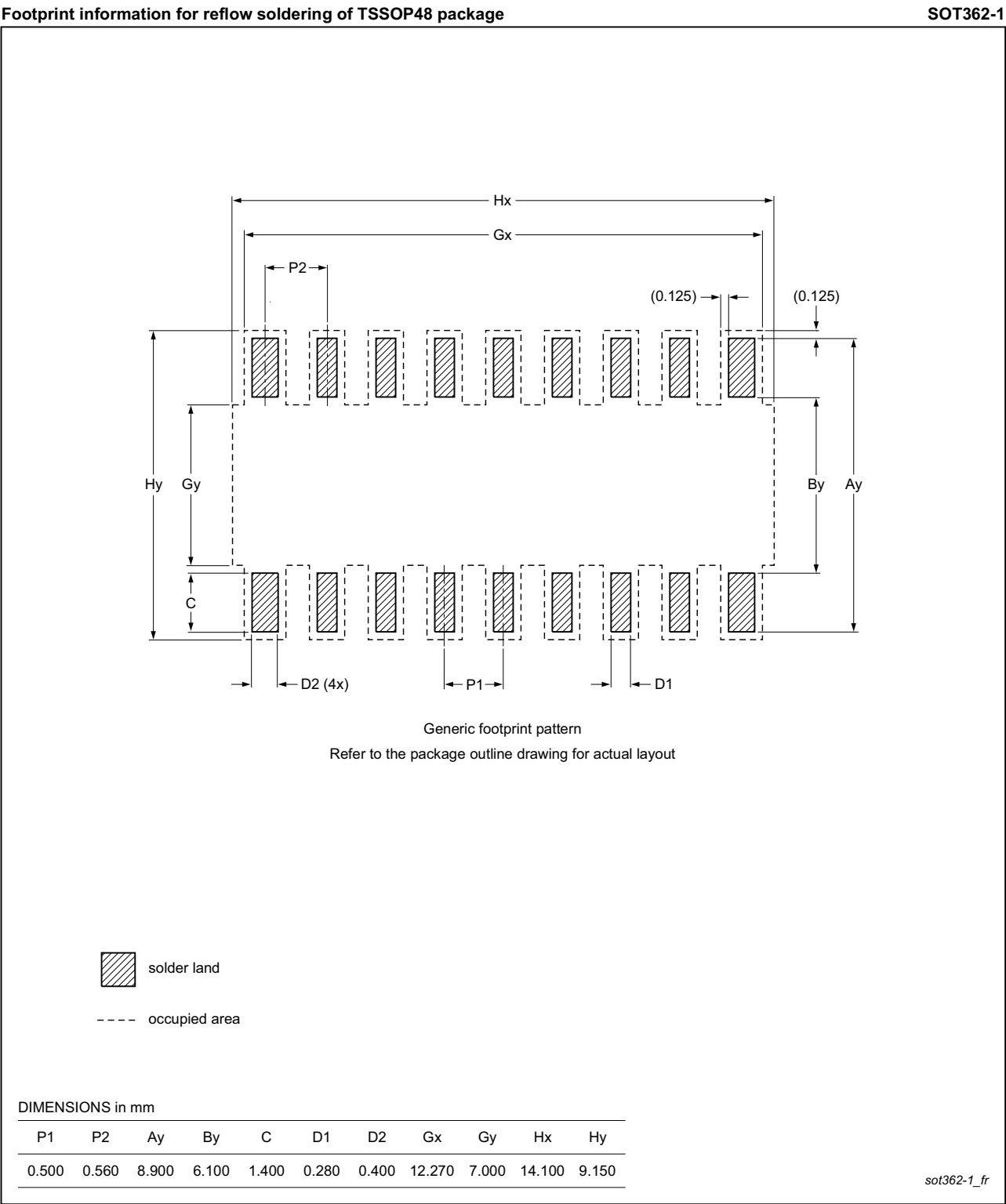
Fig 30. Footprint information for reflow soldering of SOT362-1 (TSSOP48) of PCA85262ATT
