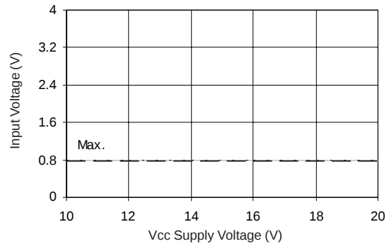
Figure 13B. Logic "0"( \overline{\text{HIN}} ) & Logic "1"( \overline{\text{LIN}} ) Input Voltage vs Voltage
