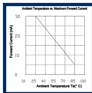
DERATING
