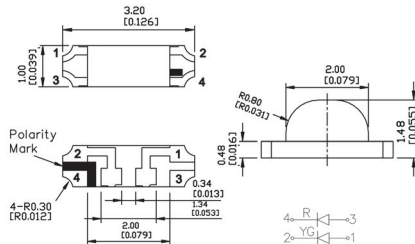
Package Outline Drawing:
