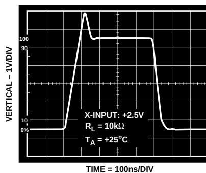
Figure 25. Y-Input Large-Signal Transient Response, C_L = 100 \text{ pF}
