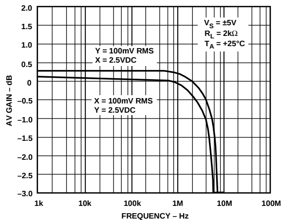
Figure 21. Gain Flatness vs. Frequency
