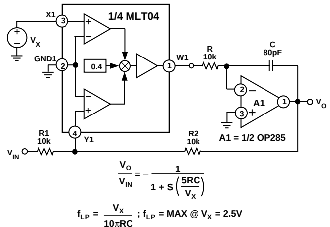
Figure 49. A Voltage-Controlled Low-Pass Filter For example, if R1 = R2 = 10 kΩ, R = 10 kΩ, and C = 80 pF,
