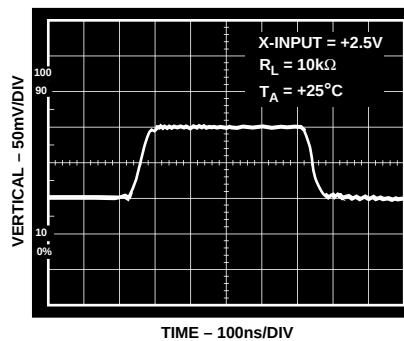
Figure 22. Y-Input Small-Signal Transient Response, C_L = 30 \text{ pF}
