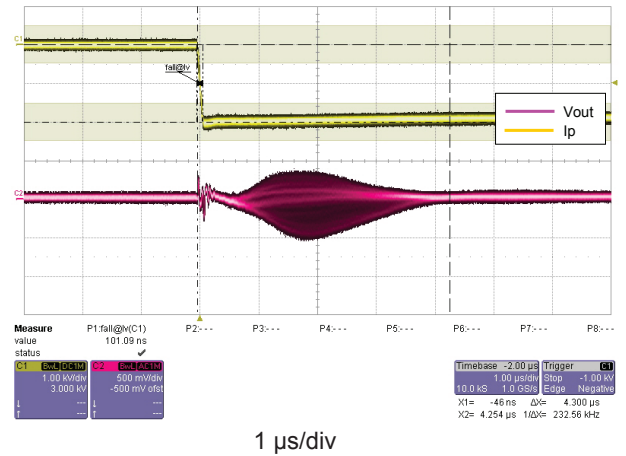
Figure 4: dv/dt
