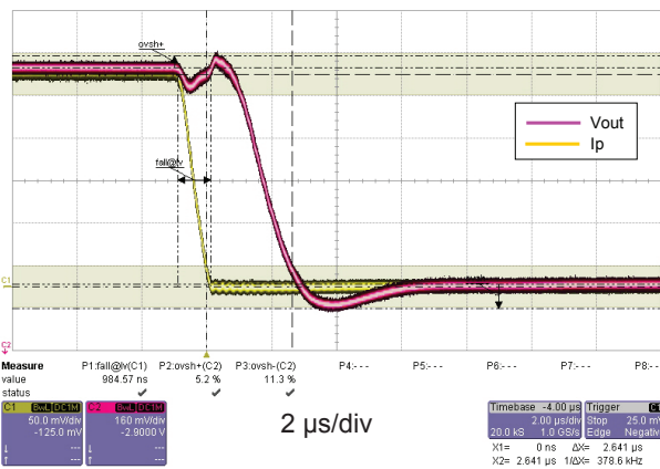
Figure 13: Step response
