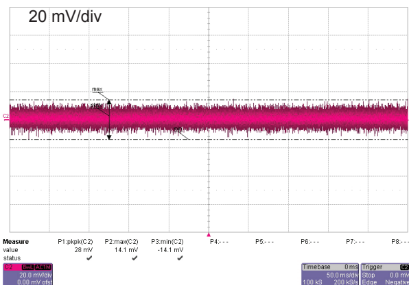
Figure 15: Output noise
