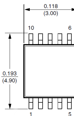
Figure 12.3 MSOP-10 Top view.
