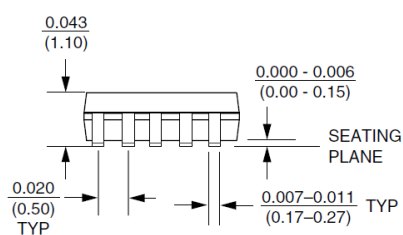
Figure 12.2 MSOP-10 Side view.
