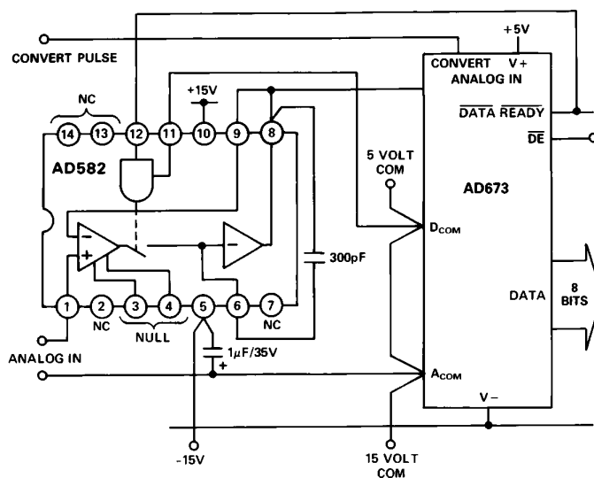
Figure 8. Sample-Hold Interface to the AD673
