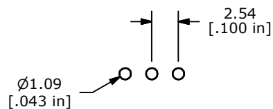
P.C. MOUNTING
