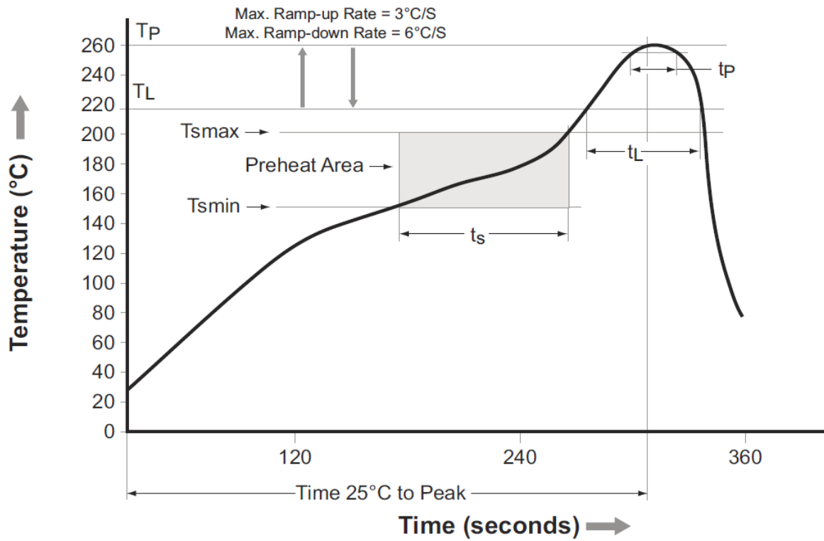
Figure 11. Reflow Profile
