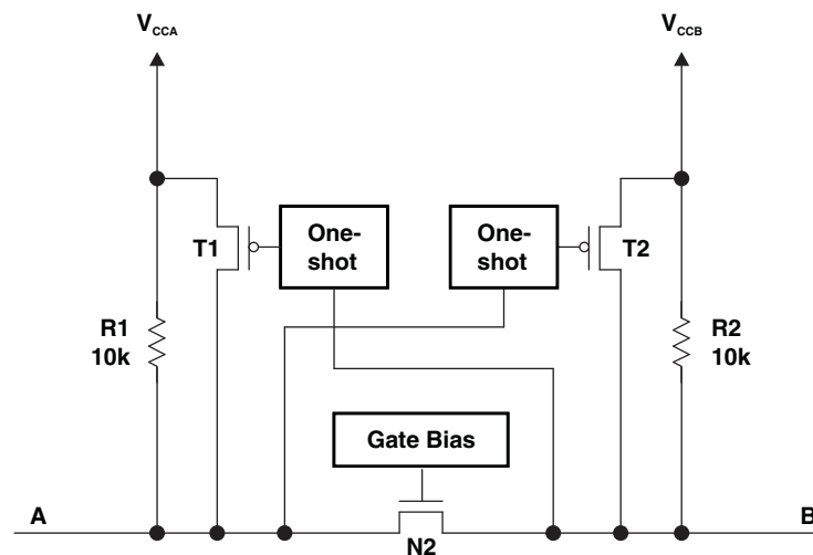
Figure 1. Architecture of a TXS01xx Cell
