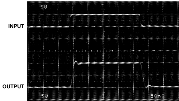
LARGE SIGNAL RESPONSE
