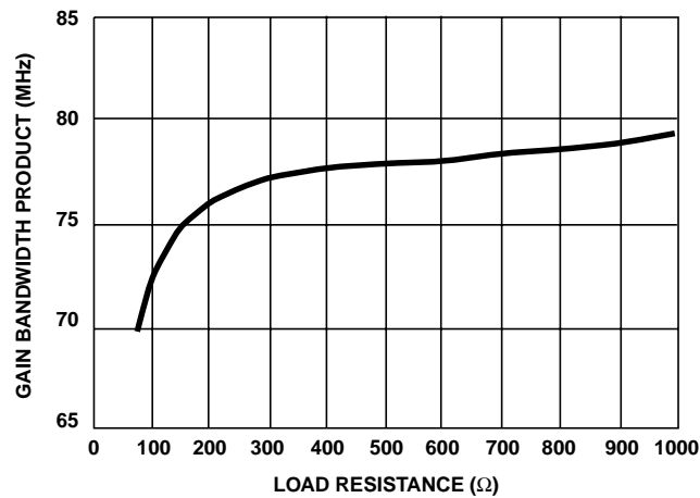
FIGURE 19. GAIN BANDWIDTH PRODUCT vs LOAD RESISTANCE
