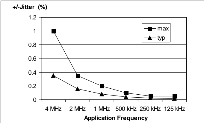
Figure 65. Integrated PLL Jitter vs signal frequency 1
