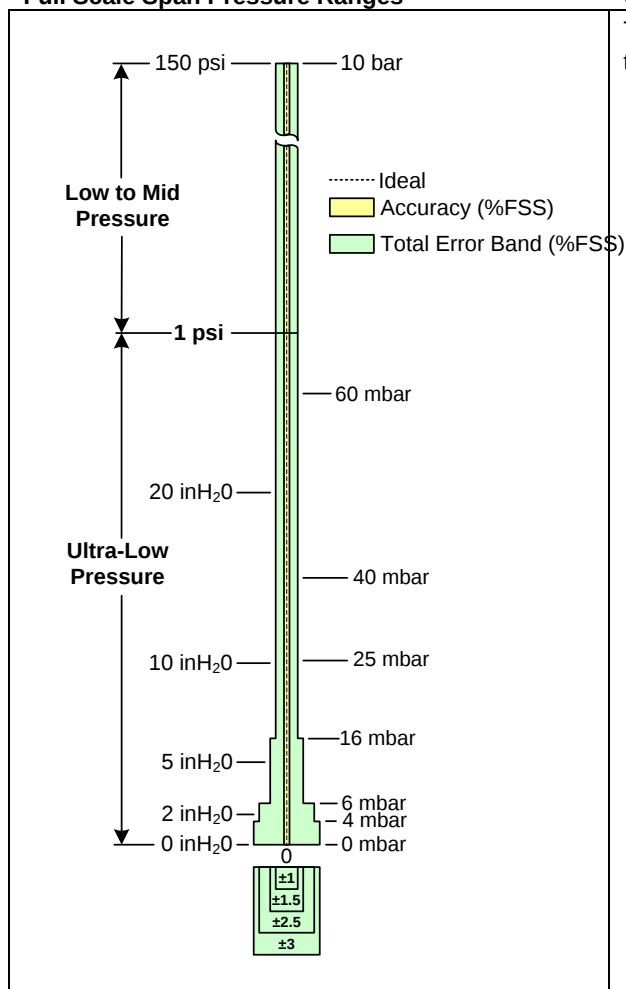
Figure 4. HSC Series Total Error Band Values for Full Scale Span Pressure Ranges
