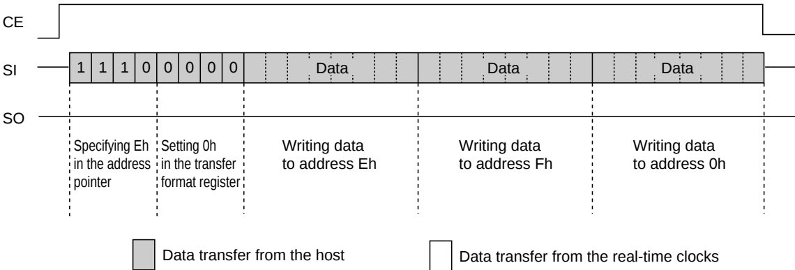
Example of Burst Writing Data Transfer (For Writing Data to Addresses Eh, Fh, and 0h)
