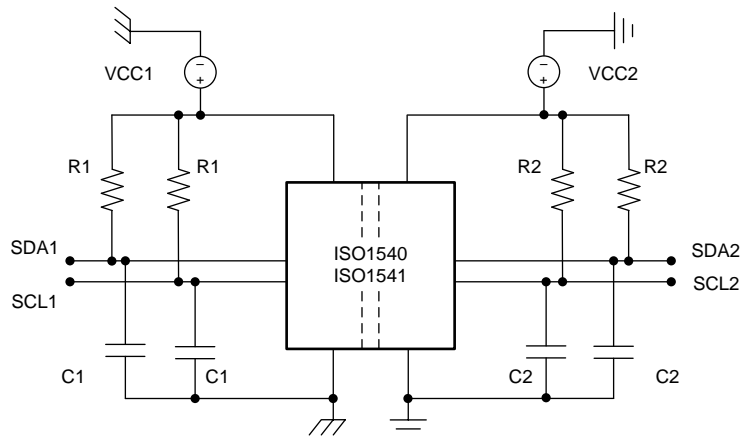
Figure 19. Test Diagram
