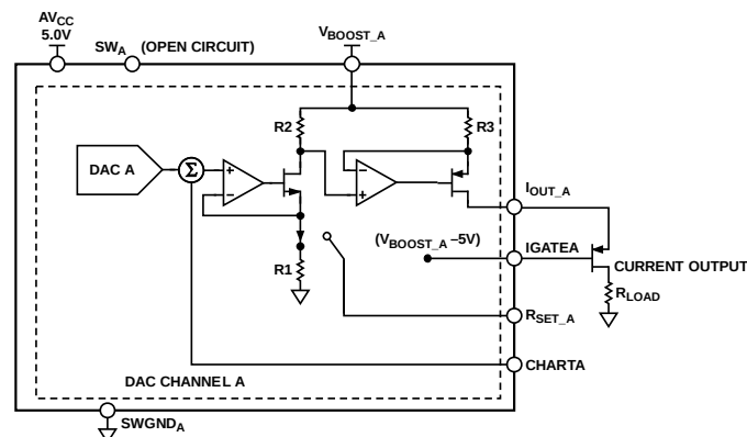
Figure 63. Configuration of a Particular Channel Using IGATE
