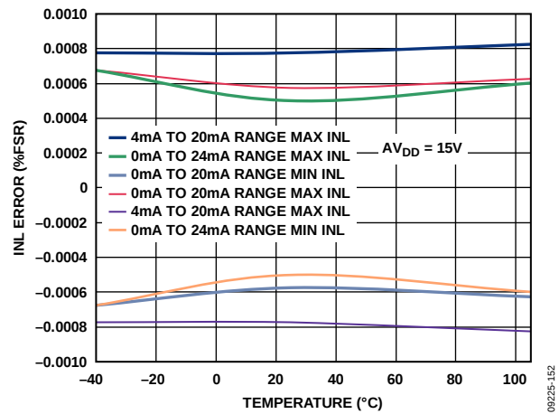
Figure 12. Integral Nonlinearity vs. Temperature, Internal R_{SET}
