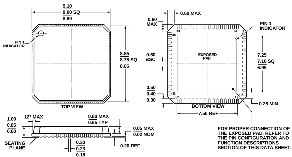
COMPLIANT TO JEDEC STANDARDS MO-220-VMMD-4 Figure 68. 64-Lead Lead Frame Chip Scale Package [LFCSP_VQ] 9 mm × 9 mm Body, Very Thin Quad (CP-64-3) Dimensions shown in millimeters
