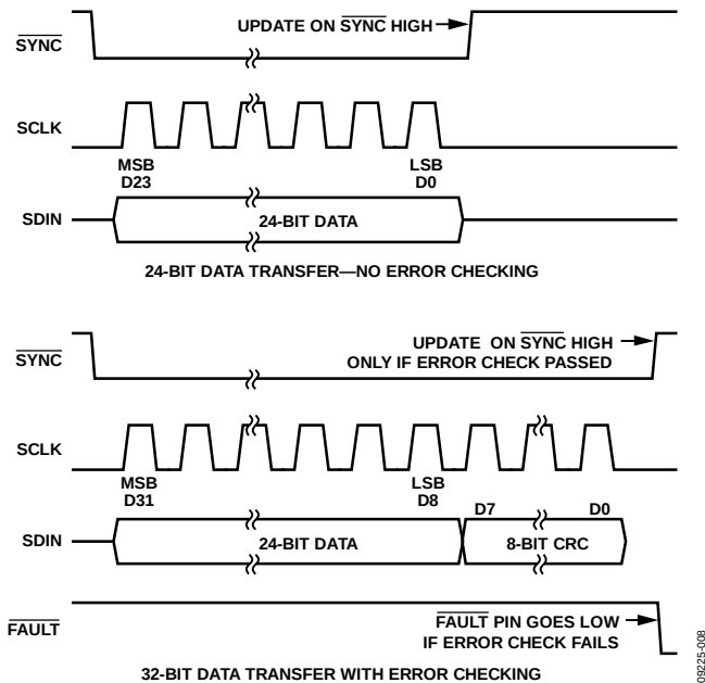
Figure 55. PEC Timing
