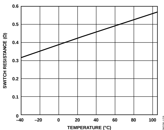
Figure 38. Switch Resistance vs. Temperature
