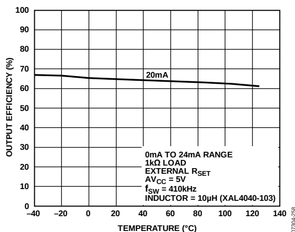
Figure 37. Output Efficiency vs. Temperature (See Figure 57)
