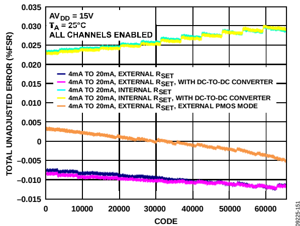
Figure 11. Total Unadjusted Error vs. Code
