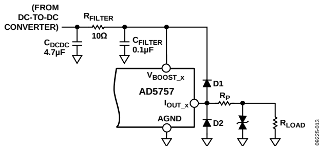
Figure 64. Output Transient Voltage Protection
