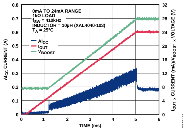
Figure 62. AI_{CC} Current vs. Time for 24 mA Step Through 1 k \Omega Load with Slew Rate Control
