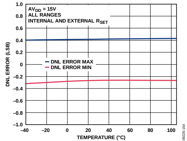
Figure 14. Differential Nonlinearity vs. Temperature
