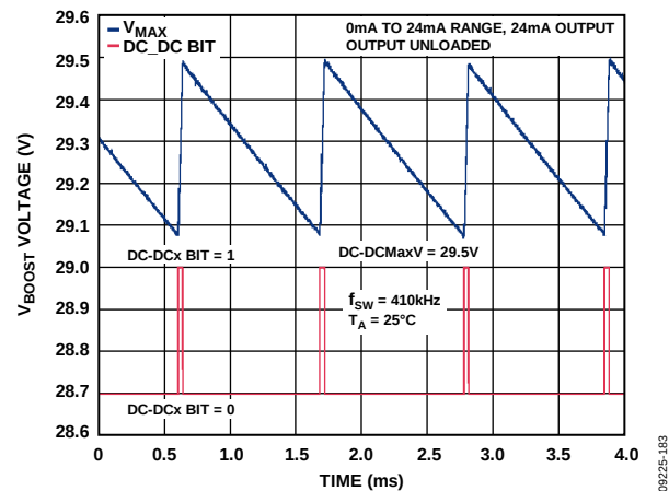
Figure 58. Operation on Reaching V_{\text{MAX}}
