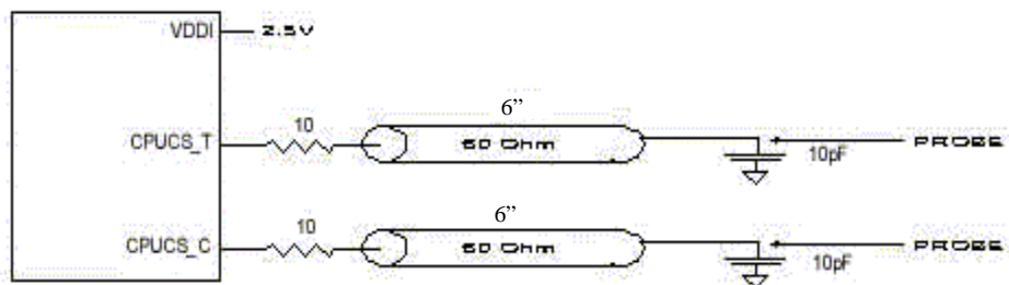
Figure 9. CS Load Termination
