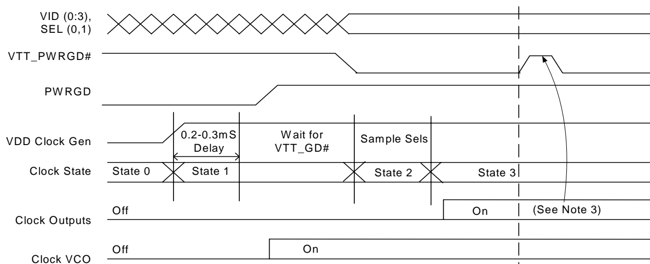
Figure 6. VTT_PWGD# Timing Diagram (with P4 Mode, SelP4 K7 = 1) [3]
