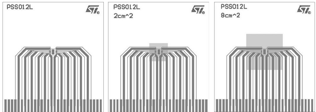
Figure 26. PowerSSO-12 PCB
