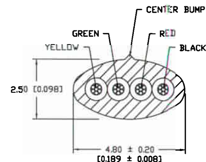
4 CONDUCTOR CABLE
