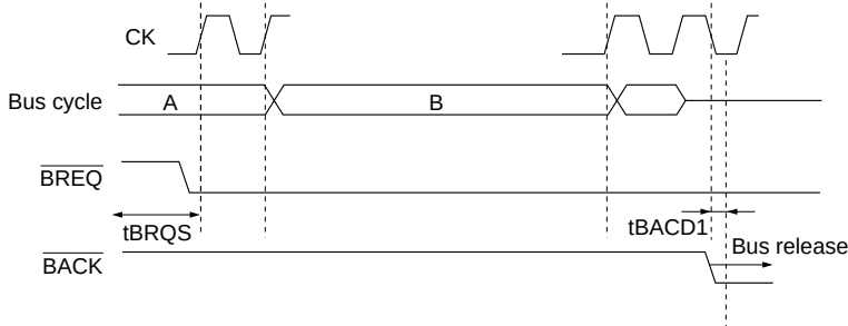
Figure 8.43 When \overline{\text{BREQ}} is Input without Satisfying t_{\text{BRQS}}
