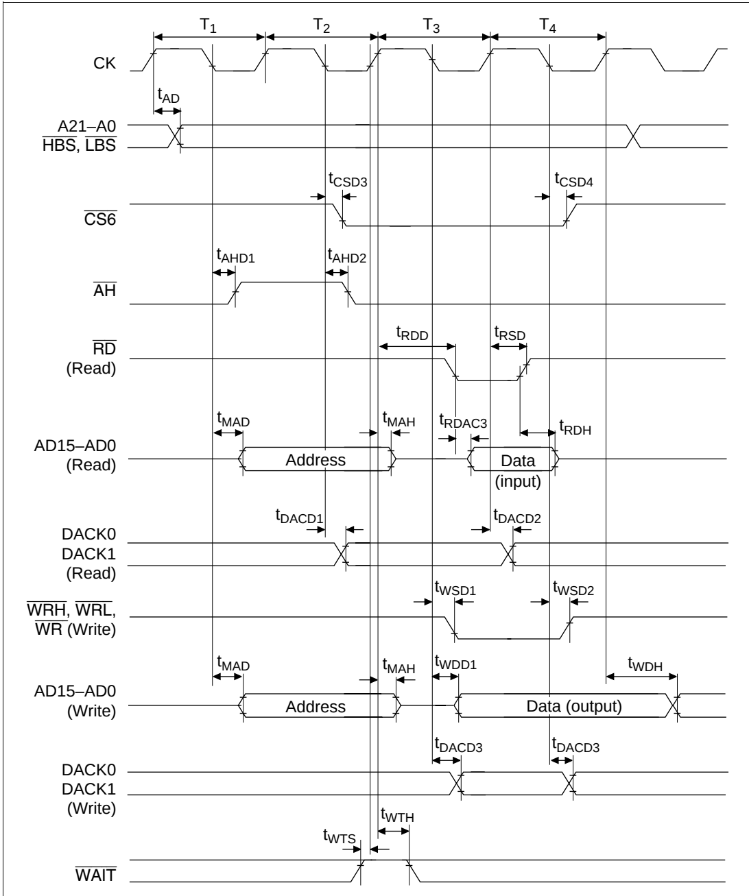
Figure 20.19 Address/Data Multiplexed I/O Bus Cycle
