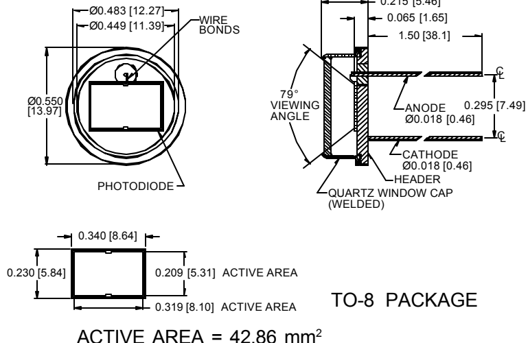
PACKAGE DIMENSIONS INCH [mm]
