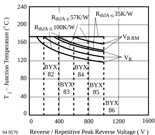
Figure 2. Junction Temperature vs. Reverse/Repetitive Peak Reverse Voltage
