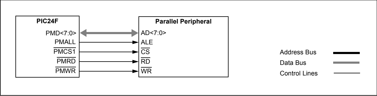
FIGURE 19-10: PARALLEL EEPROM EXAMPLE (UP TO 15-BIT ADDRESS, 8-BIT DATA)
