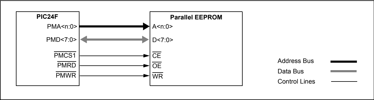
FIGURE 19-11: PARALLEL EEPROM EXAMPLE (UP TO 15-BIT ADDRESS, 16-BIT DATA)
