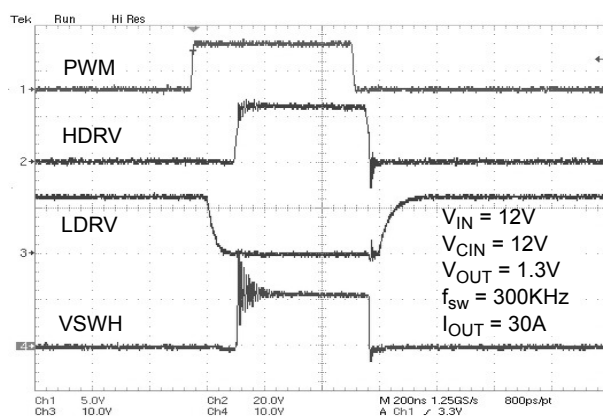
Figure 21. Switching Waveform at I_{OUT} = 30A
