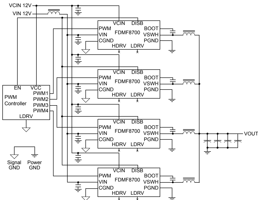
Figure 26. Typical Application
