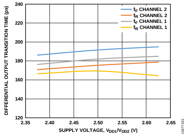
Figure 25. Differential Output Transition Time vs. Supply Voltage, V_{DD1}/V_{DD2}
