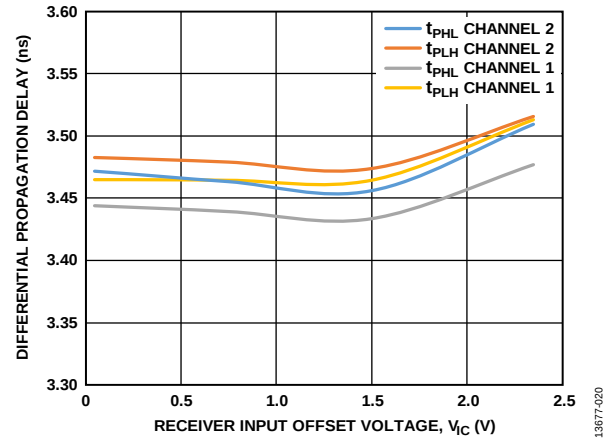
Figure 24. Differential Propagation Delay vs. Receiver Input Offset Voltage, V_{IC}
