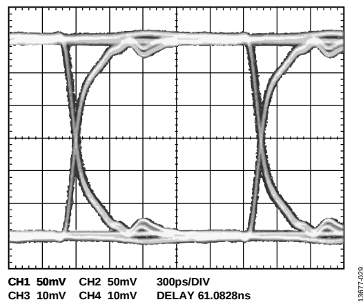
Figure 33. ADN4651 Eye Diagram for D_{OUT2\pm}
