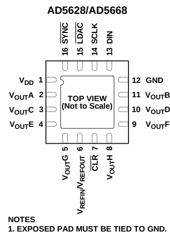
Figure 5. 16-Lead LFCSP (CP-16-17)
