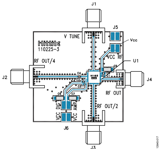
Figure 17. Evaluation PCB
