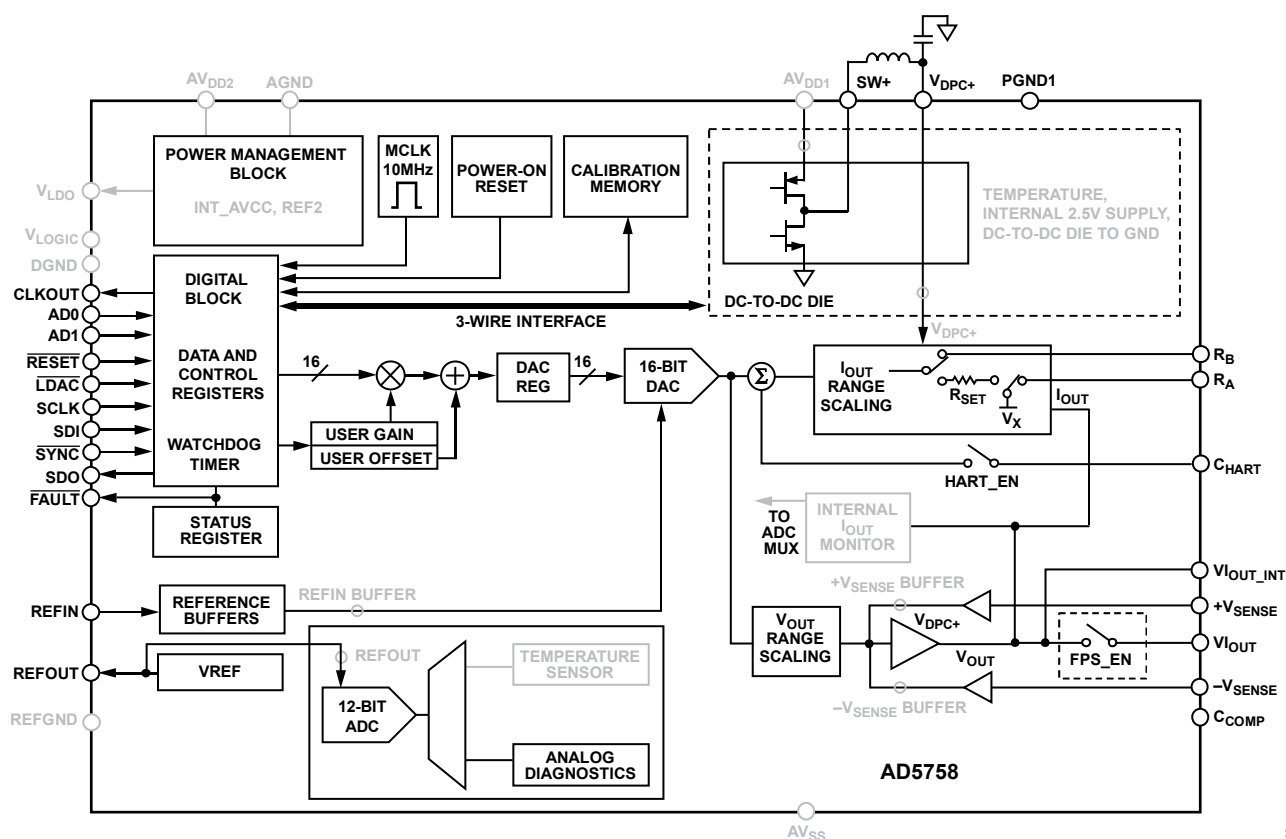
Figure 85. Diagnostic ADC Input Nodes
