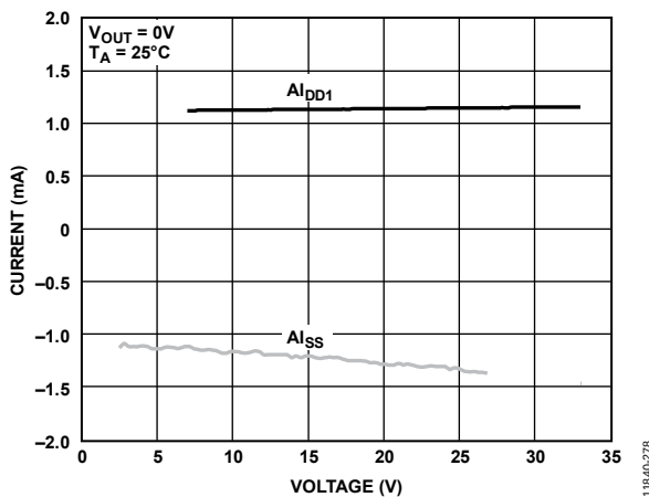
Figure 69. I_{\text{DD1}}/I_{\text{SS}} Current vs. A_{\text{VDD1}}/|A_{\text{VSS}}| Supply
