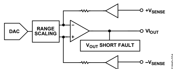
Figure 75. Voltage Output
