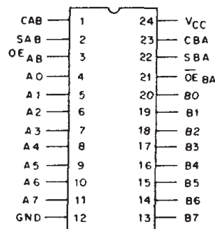
TERMINAL ASSIGNMENT
