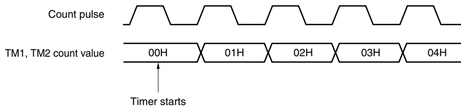
Figure 9-11. Start Timing of 8-Bit Timer Counter
