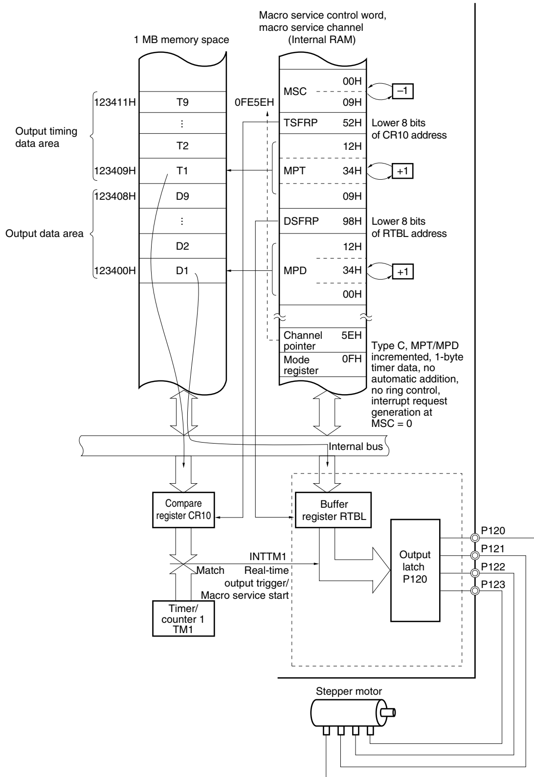
Figure 22-32. Stepper Motor Open Loop Control by Real-Time Output Port
