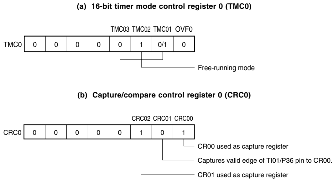
Figure 8-13. Control Register Settings for Measurement of Two Pulse Widths with Free-Running Counter
