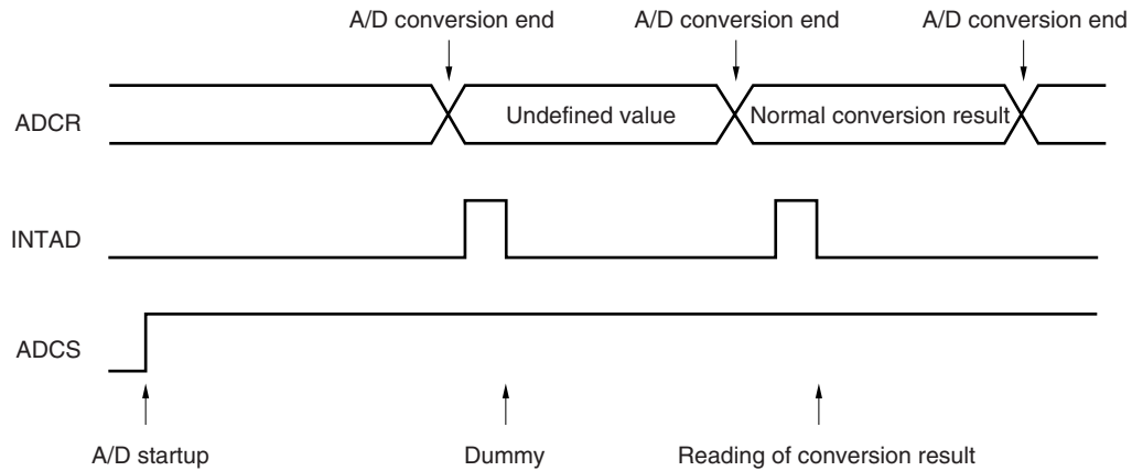
Figure 13-17. Conversion Results Immediately After A/D Conversion Is Started
