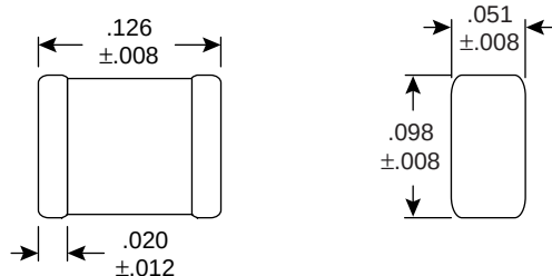
Dimensions (In.)
