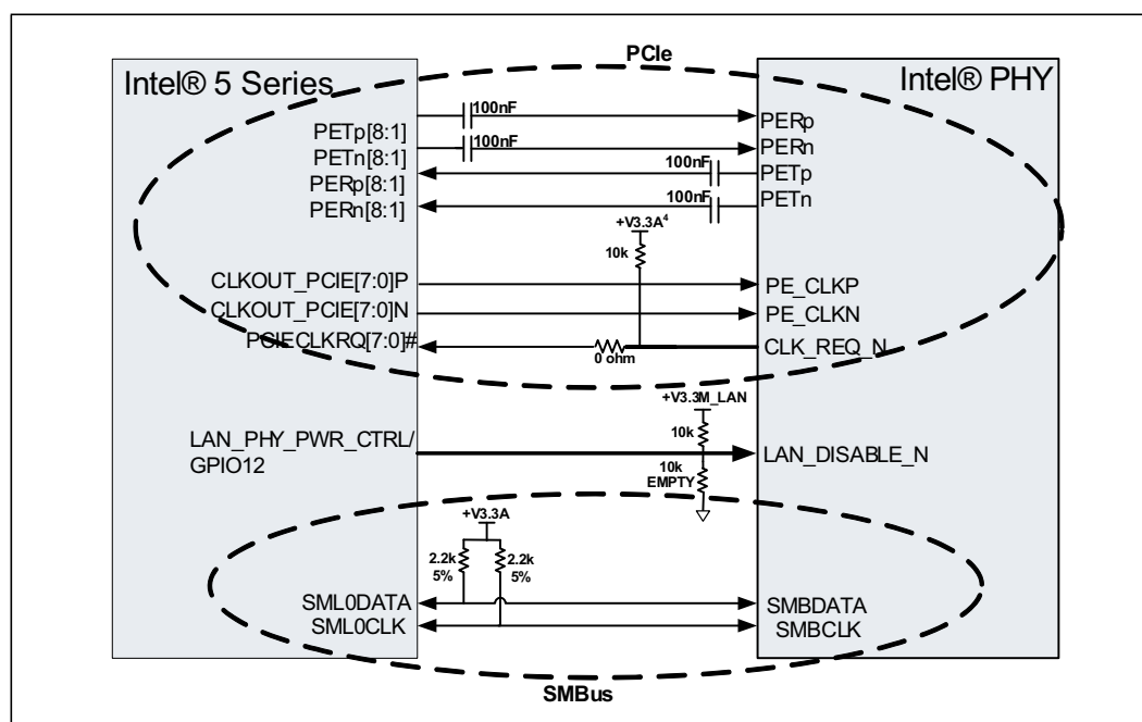
Figure 2. Intel® 5 Series Express Chipset / 82577 Interconnects
