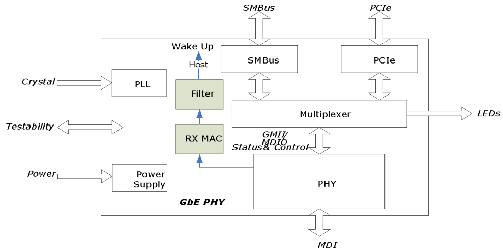
Figure 1. 82577 Block Diagram
