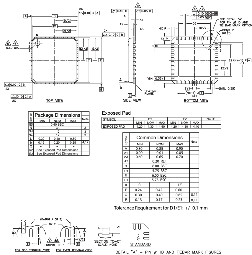
Figure 3. Package Dimensions
