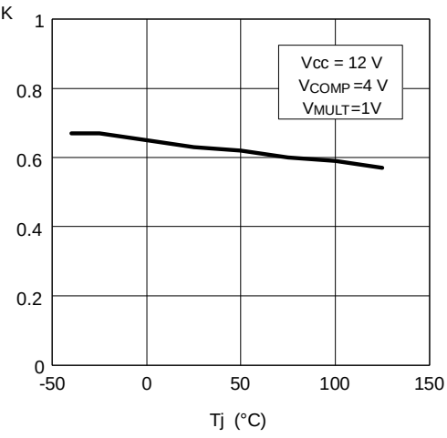
Figure 13. Multiplier gain vs. T_j
