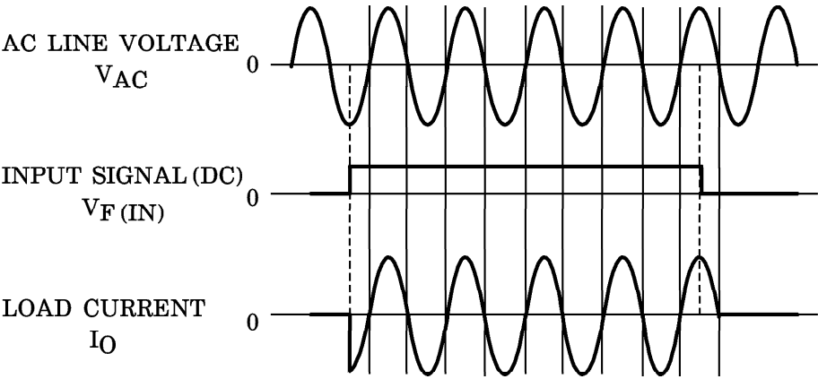
Fig. 1. SWITCHING WAVEFORM
