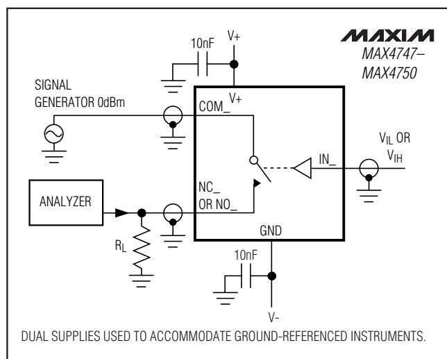
Figure 5. Off-Isolation/On-Channel Bandwidth
