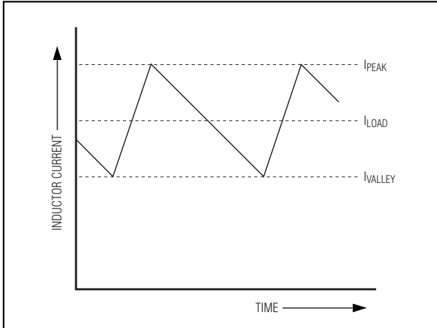
Figure 4. Inductor-Current Waveform
