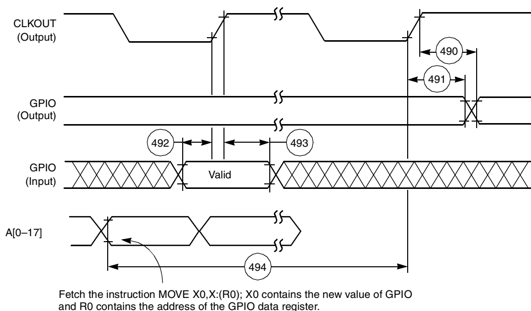
Figure 2-34. GPIO Timing
