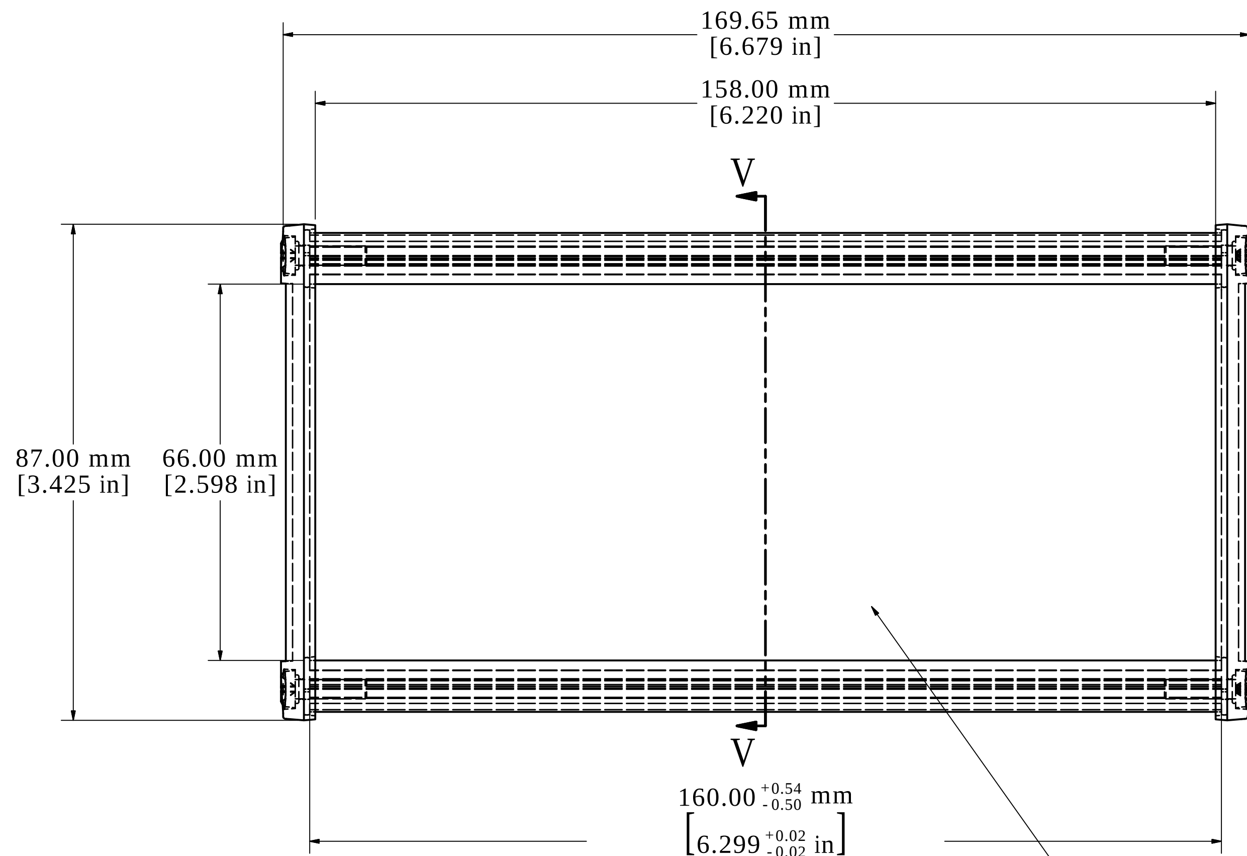
ASSEMBLY - VIEW FROM TOP
