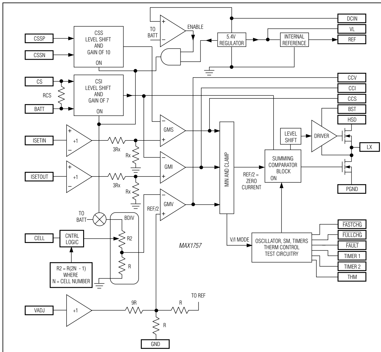
Figure 3. Functional Diagram
