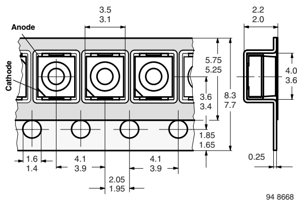
Figure 8. Tape dimensions in mm for PLCC-2
