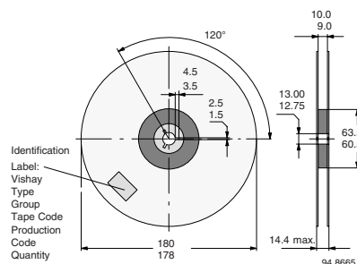
Figure 9. Reel dimensions - GS08
