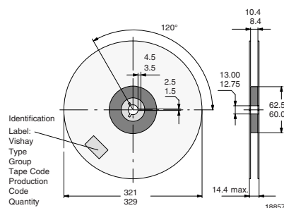
Figure 10. Reel dimensions - GS18
