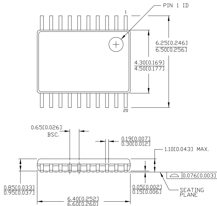
Figure 5. 20-LD TSSOP, Thin Shrunk Small Outline Package (4.40 mm Body) ZZ2
